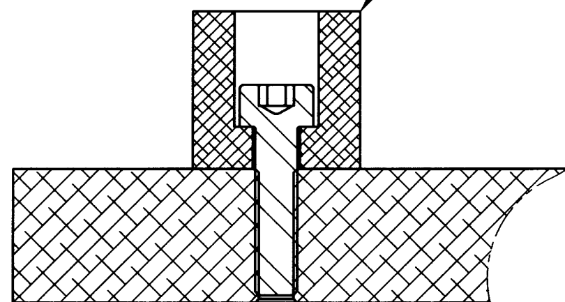
SECTION Y-Y (SOME DETAILS NOT SHOWN FOR CLARITY) SCALE 2 : 1
