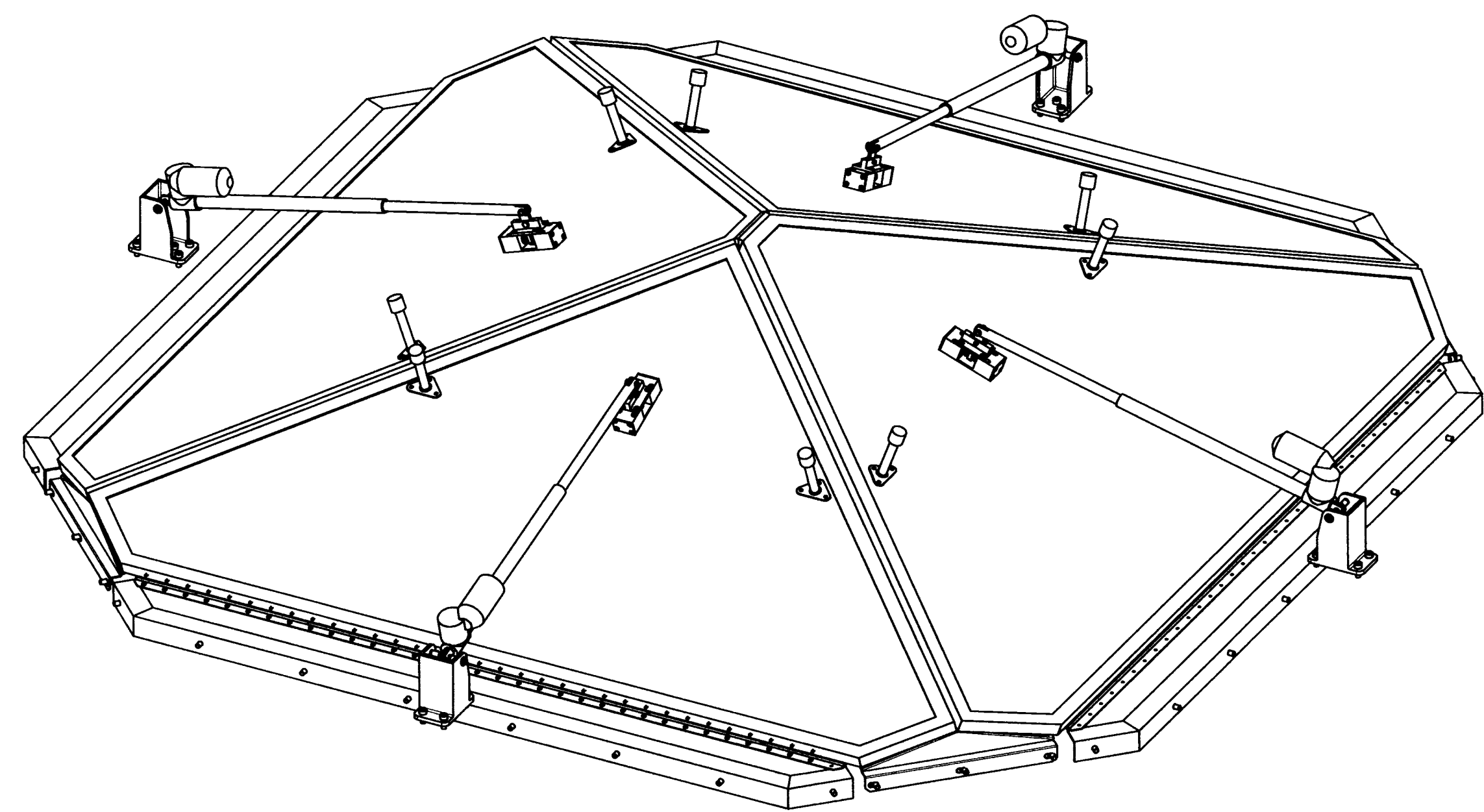
VIEW SHOWING ALL FOUR DOORS CLOSED
