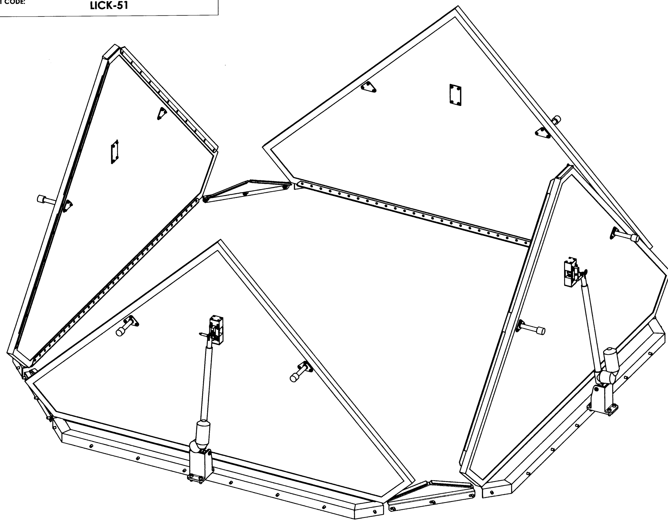
VIEW SHOWING DOORS OPEN
