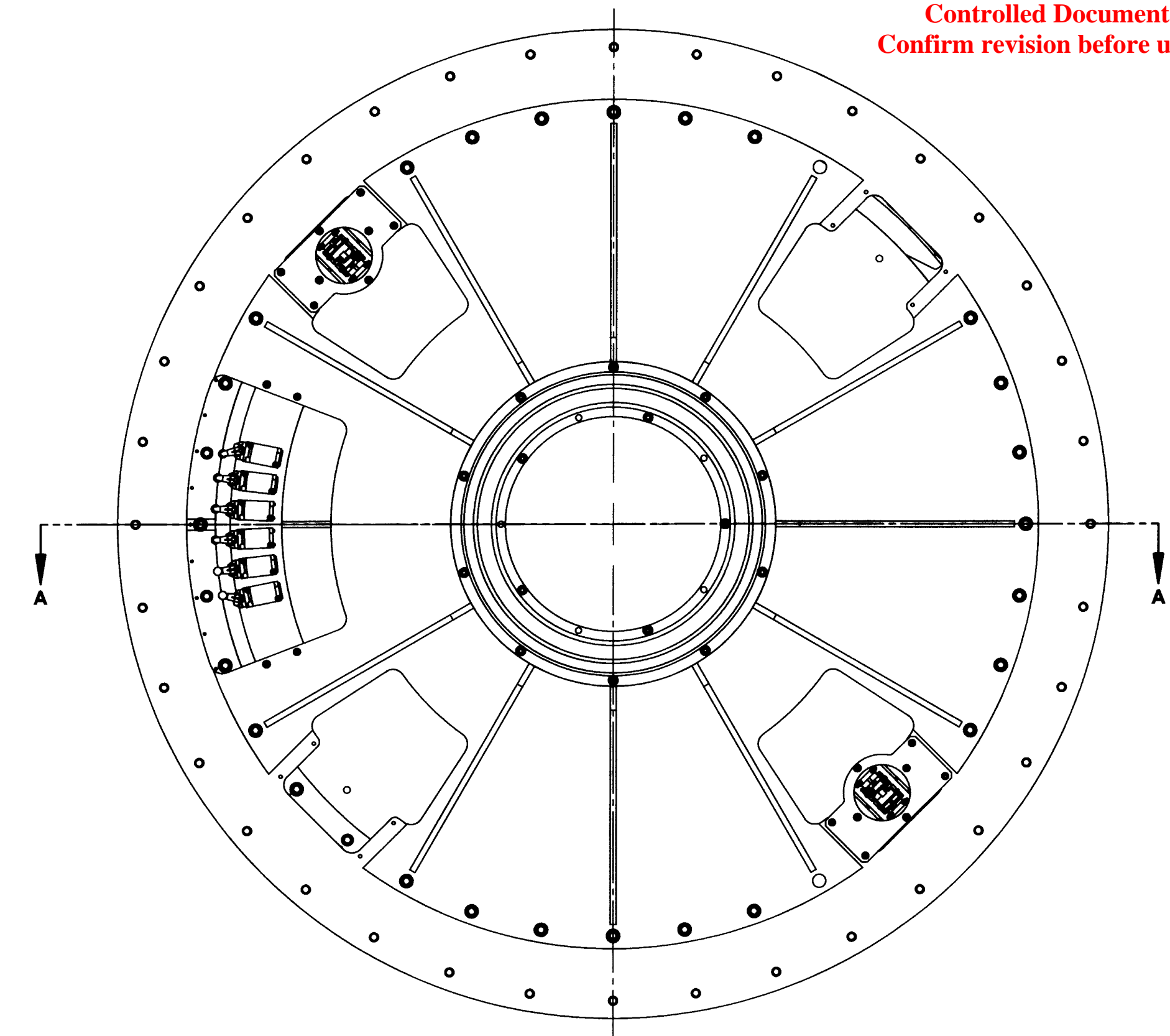
BOTTOM VIEW OF DIRECT DRIVE ASSEMBLY
