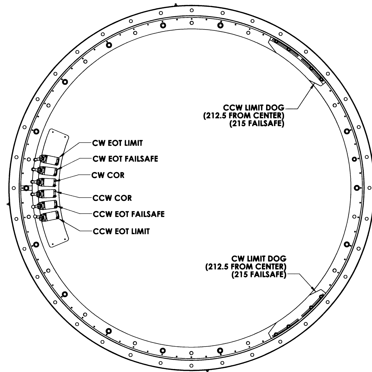
BOTTOM VIEW OF LIMIT SWITCH ASSEMBLY AND ENCODER RING
