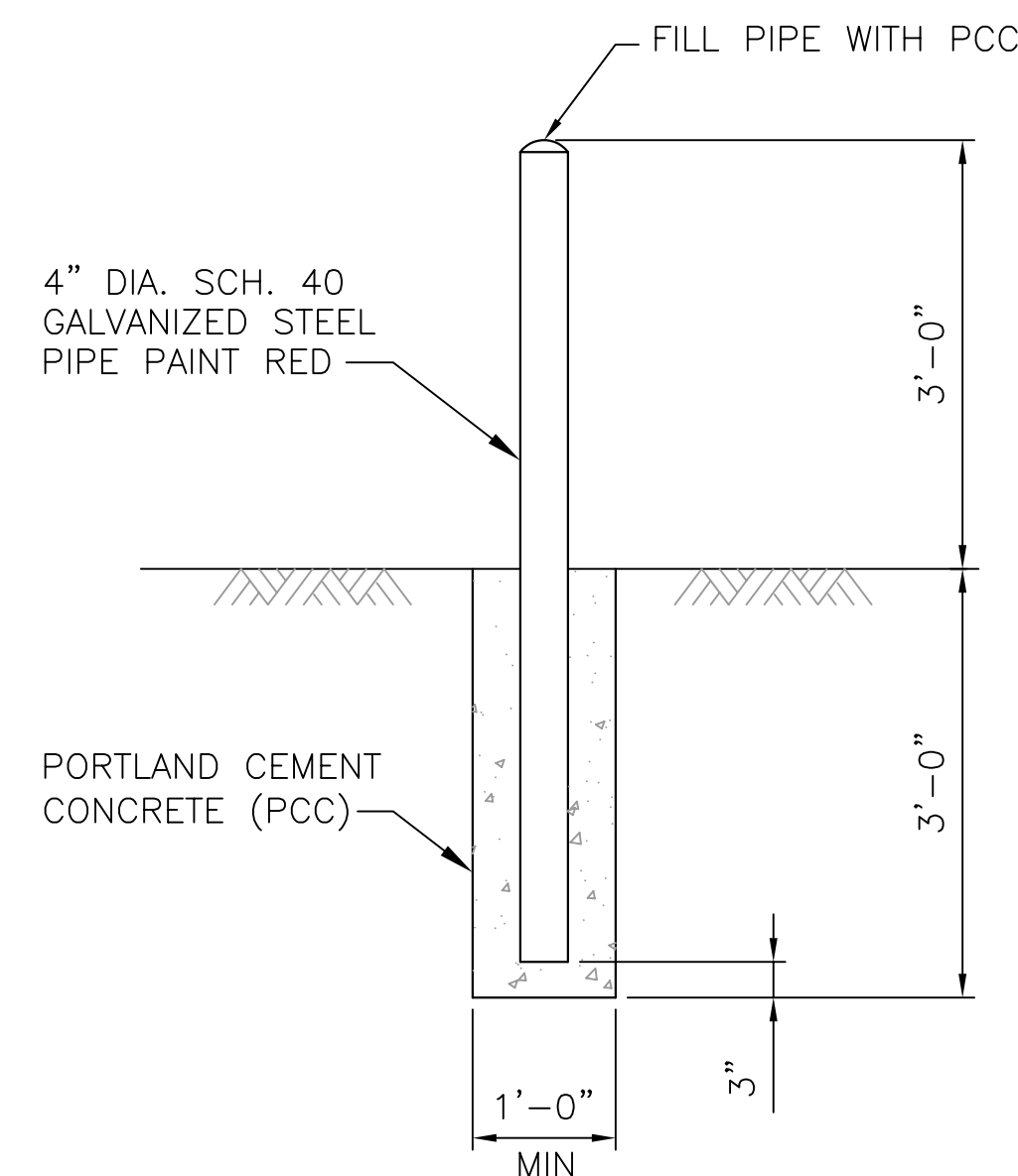
FIXED GUARD POST 1 SCALE: NTS
