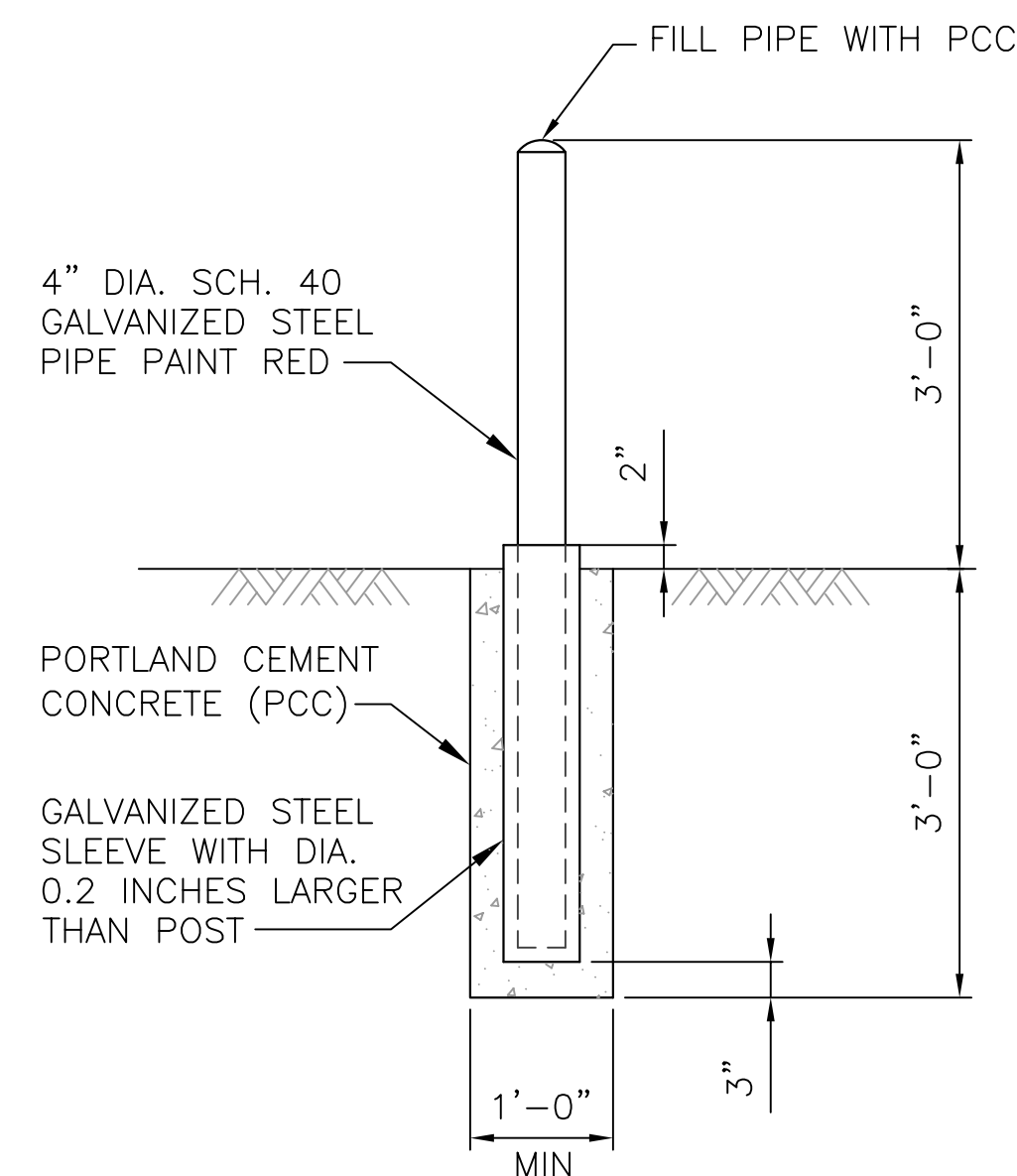
REMOVEABLE GUARD POST 2 SCALE: NTS
